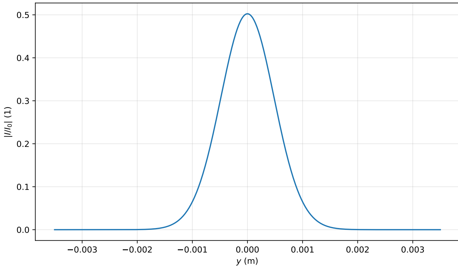
Intensity profile I(x=0, y, z=2.149)/I_0 , \text{Pin}=0.1\text{Pcr} , artificial time
